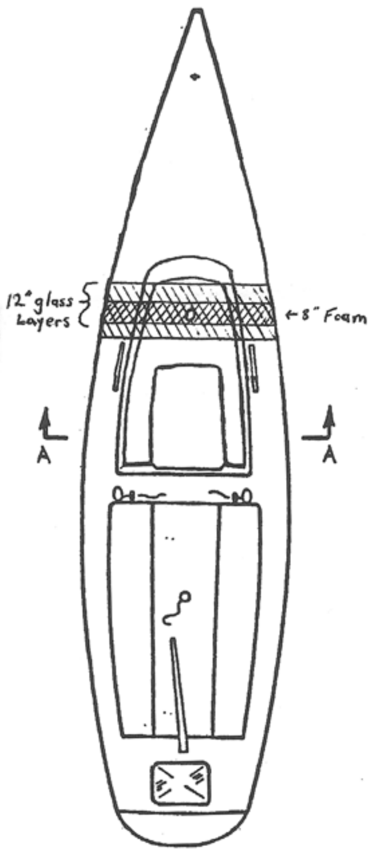
FIGURE 2 SKETCH OF Mast Step Lay up REINFORCEMENT
